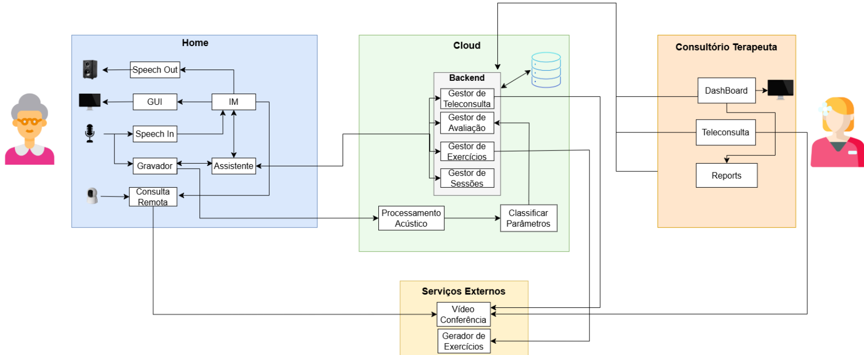
Fig.3: Arquitetura Speech Therapy at Home
